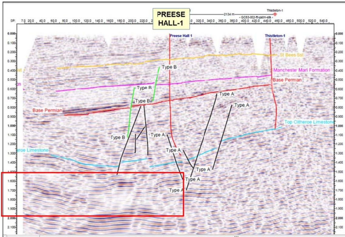
Figure XI-4: Seismic Reflection Line Showing Suspected Active Faults Near The Preese Hall-1 Well In The Bowland Sub-basin
